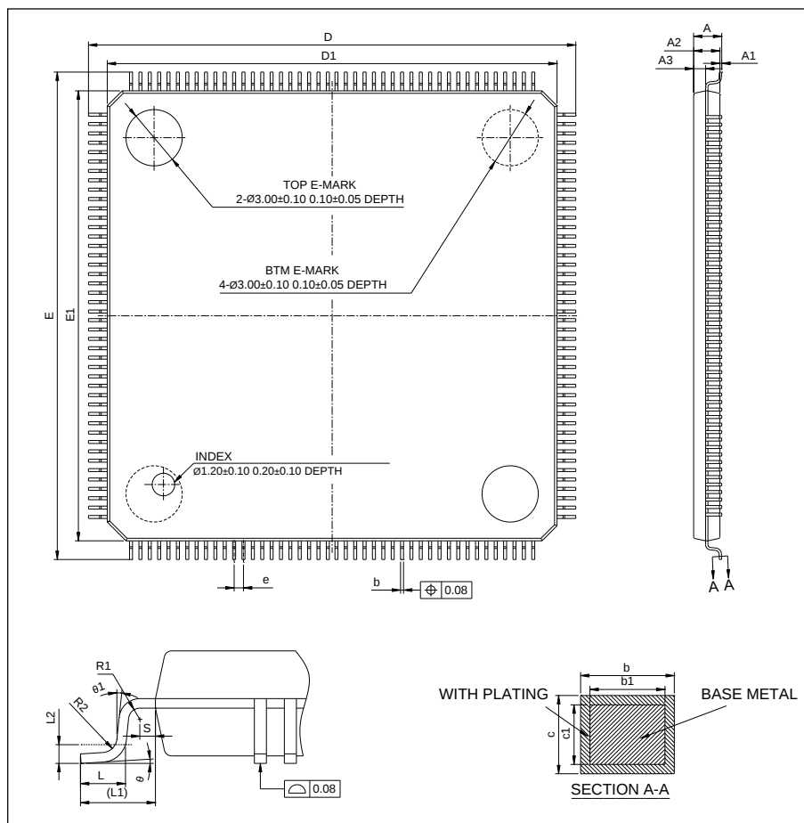
Figure 5-1. LQFP176 package outline
