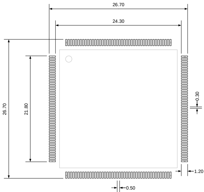
Figure 5-2. LQFP176 recommended footprint
