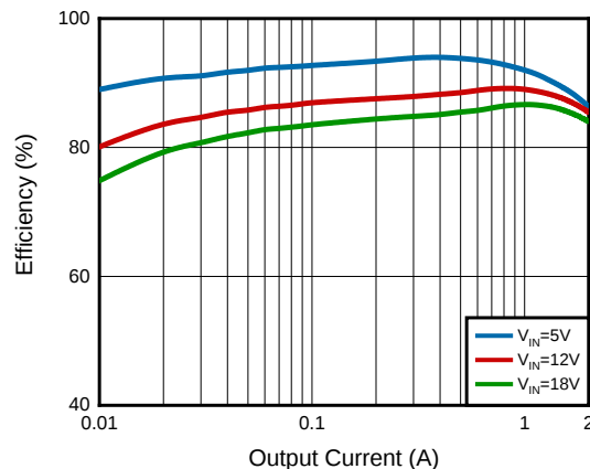
Figure 12. 3.3V Output Efficiency(DCR=27.3mΩ)
