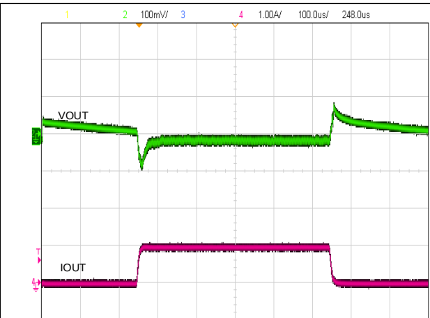
Figure 30. Load Transient
