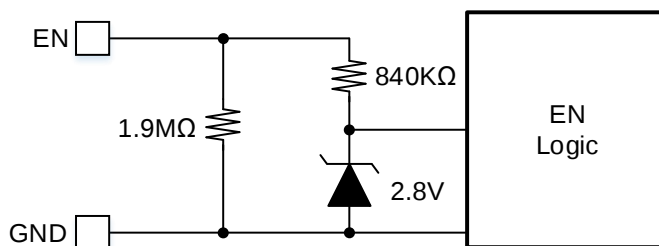
Figure 8. Zener Diode between EN and GND
