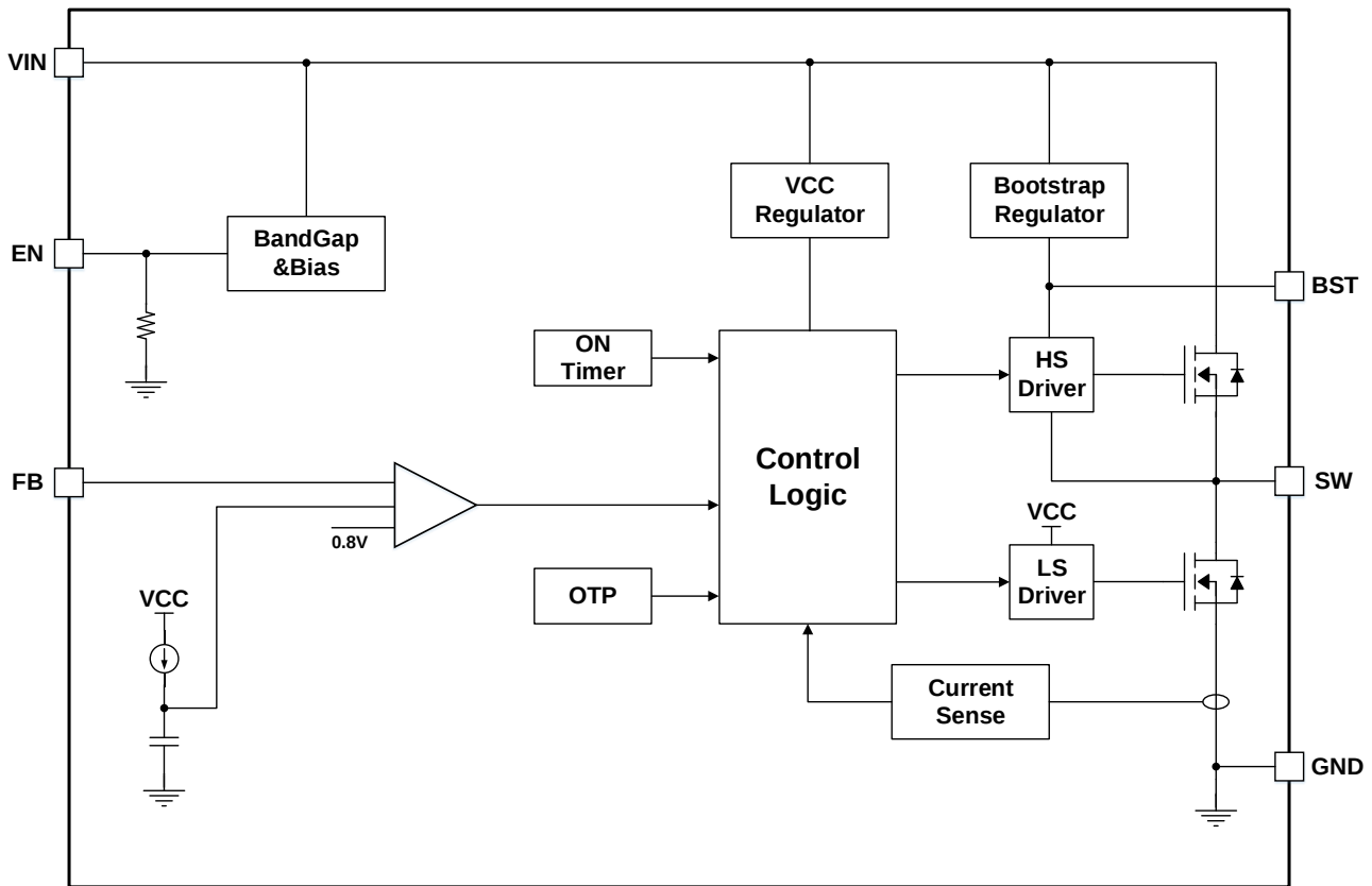
Figure 7. GD30DC1310-I06 Functional Block Diagram
