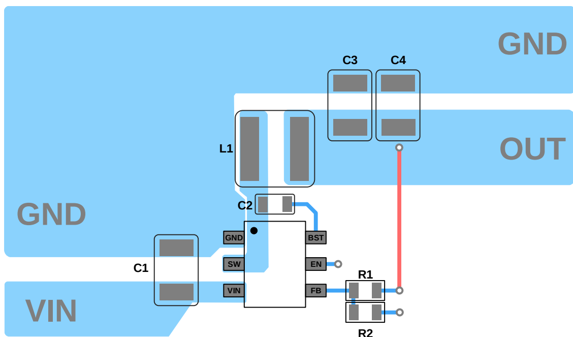
Figure 32. Typical GD30DC1310-I06 Example Layout
