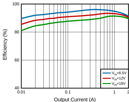
Figure 11. 5.0V Output Efficiency(DCR=20.4mΩ)
