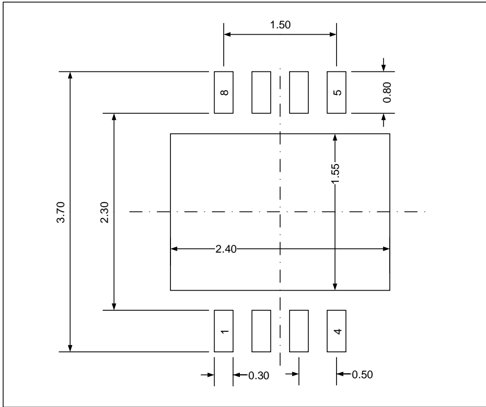
Figure 9-2 DFN8 recommended footprint
