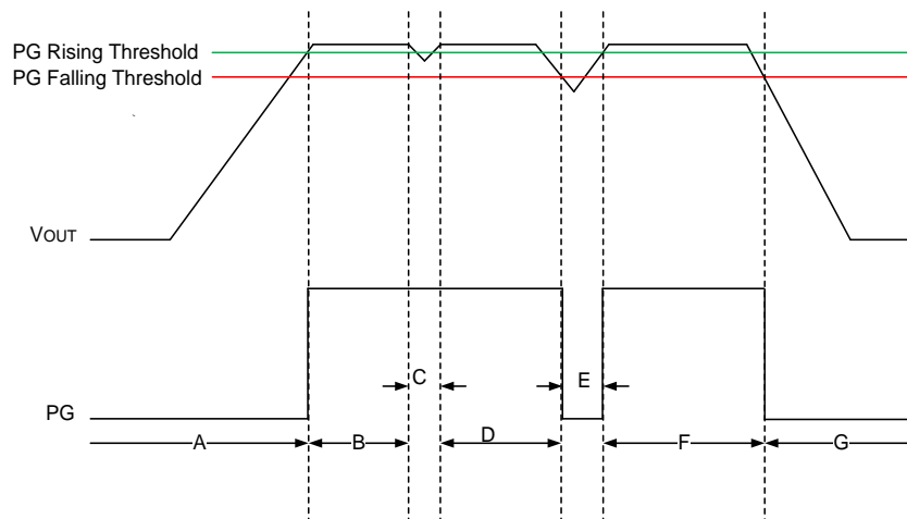
Figure 5-1 Typical PG Operation
